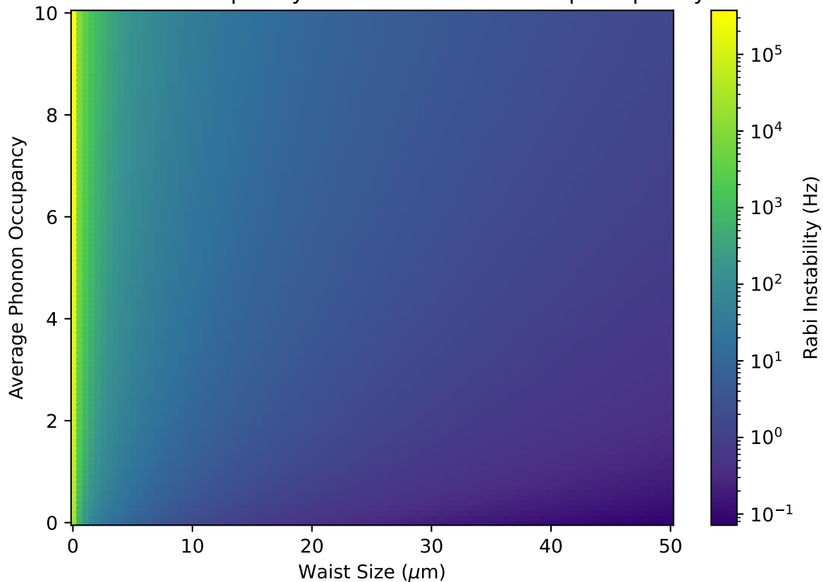
On-Axis Rabi Frequency Deviation for 1MHz Trap Frequency
